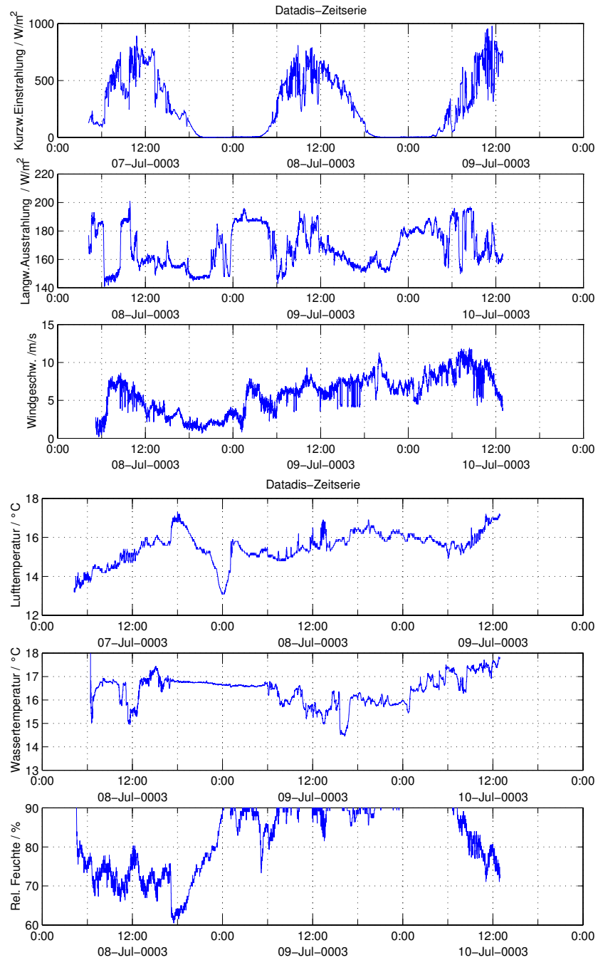
Figure 4.6: Time series of meteorological parameters. From upper to lower: shortwave radiation, long wave radiation, wind speed, air temperature, sea surface temperature, rel. humidity.
